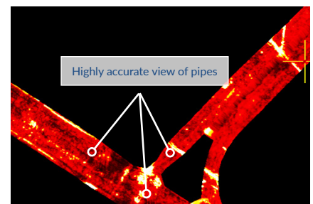
GREED HD 3D CAD: subsurface time slice view
